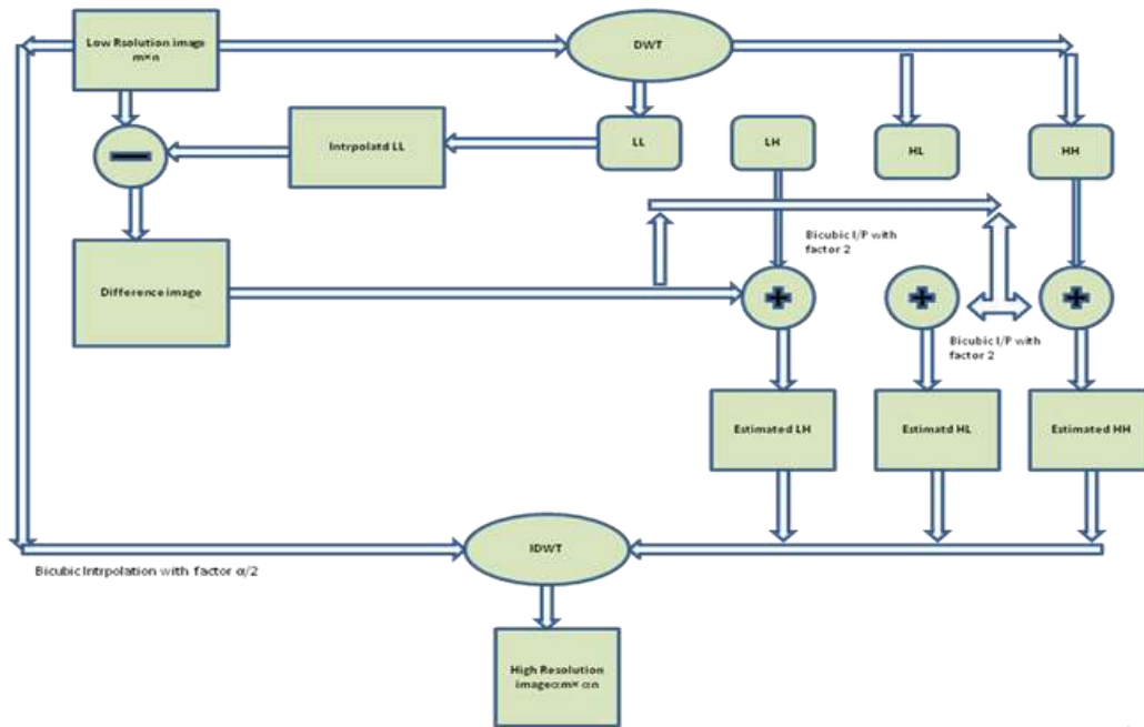
Fig. 2: Block Diagram of the Proposed Resolution Enhancement Algorithm
