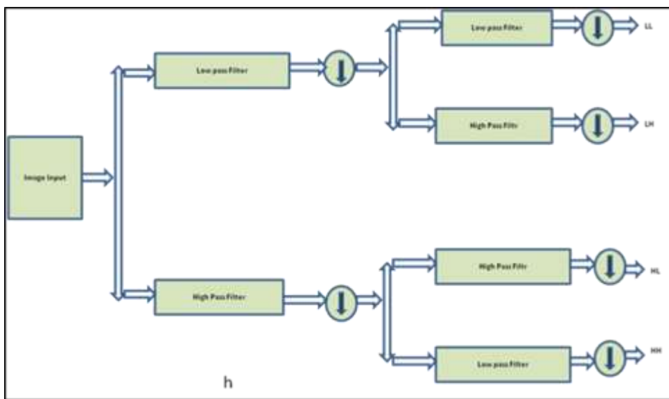
Fig. 1: Block Diagram of DWT Filter Banks of Level1
