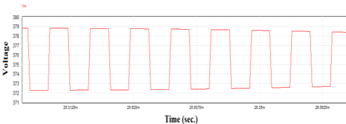
Figure 4.9. Output voltage from the wind turbine generator after converter
