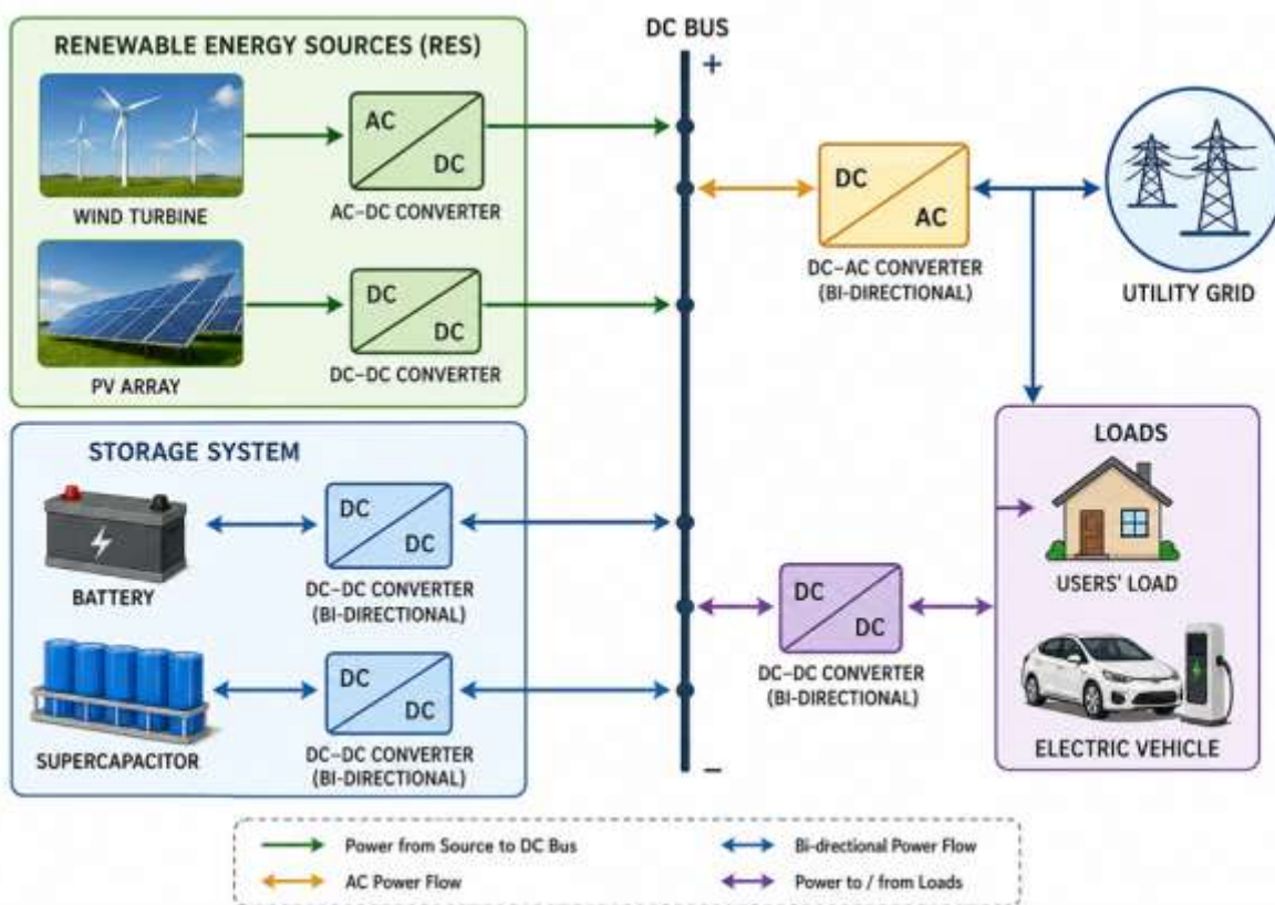
Figure 2.1 Structure of Hybrid Energy Storage System.
