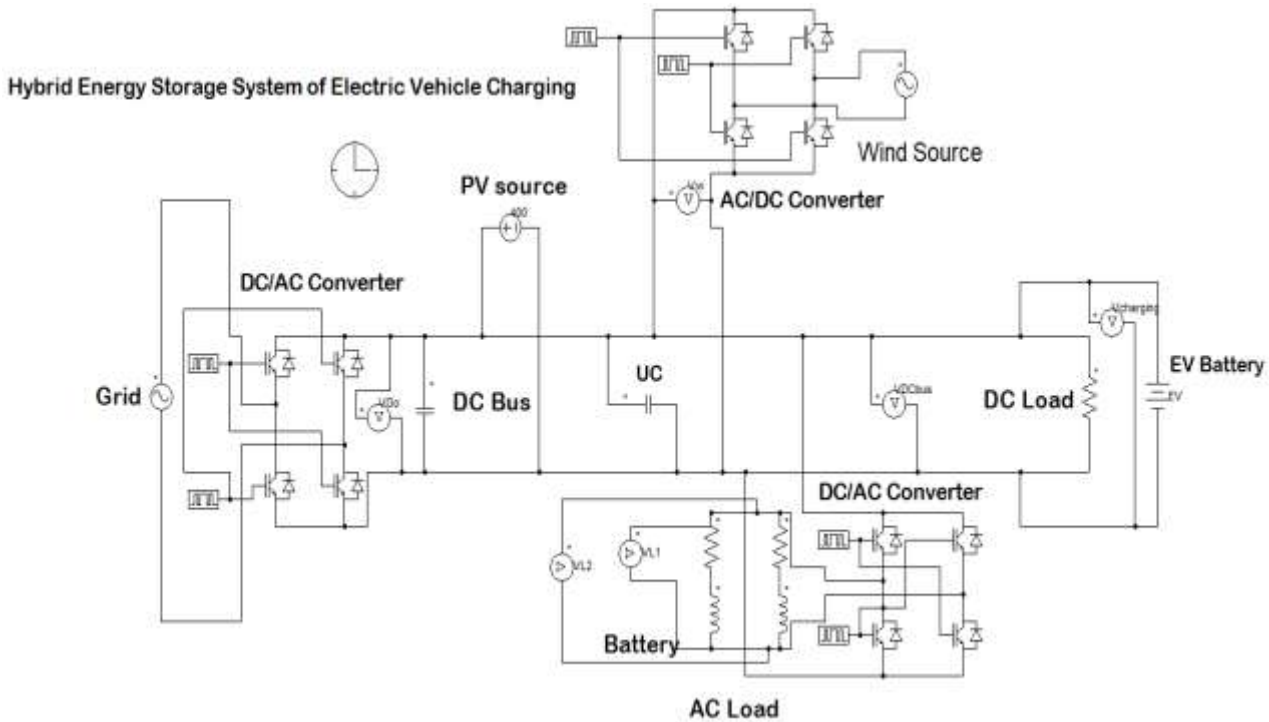
Figure 3.1: Circuit Diagram of proposed HESS for EV charging
