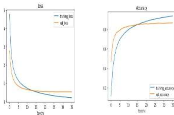
Figure 4: Visualising the loss and accuracy curve
